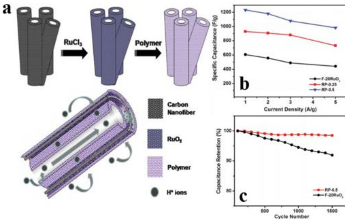
Fig. 7. (a) Schematic illustration of the synthesis of dual-wall carbon nanofibre- \text{RuO}_2 -poly(benzimidazole) (PBI) (CNFs- \text{RuO}_2 -PBI). (b) Specific capacitance of F-20RuO 2 , RP-0.25, RP-0.5 at different current densities (1 to 5 A/g). (c) Stability performance of RP-0.5 and F-20RuO 2 over 1500 cycles at current density 1 A/g [113].
