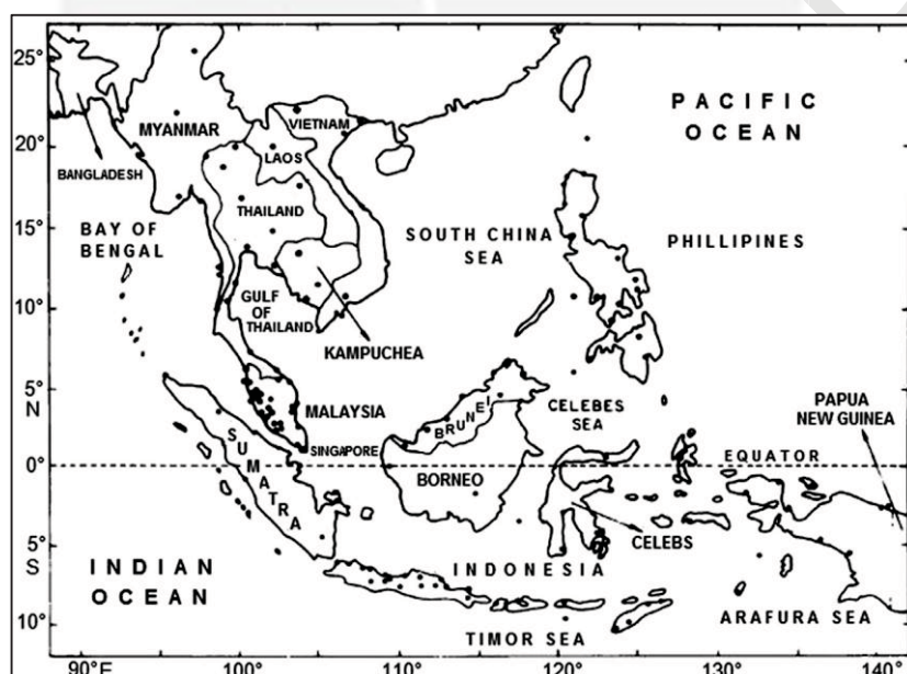
Figure 1.3: Southeast Asia region (Kripalani and Kulkarni, 1997).
