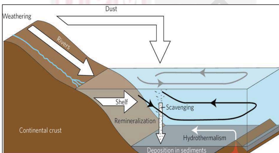
Figure 1.2: Diagram of dissolved and particulate trace metals origins in seawater which include rivers, shelf sediment and dust, but less impact from hydrothermal inputs. After the trace metals reach the sea water, biogeochemical cycling occurs, and causes vertical transport and fractionation from surface to bottom waters. In addition, the metals are distributed or transported by the water circulation (Frank, 2011).
