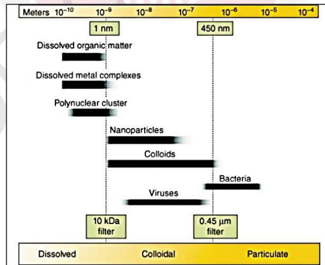
Figure 1.1: Sizes for various fractions in natural water sample and the typical constituents of the fractions. Typical filtrations use either a 0.2 or 0.45 \mu\text{m} pore size.
