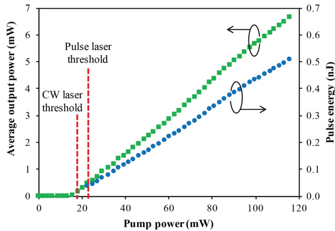
Figure 15. Average output power and pulse energy as a function of pump power.
