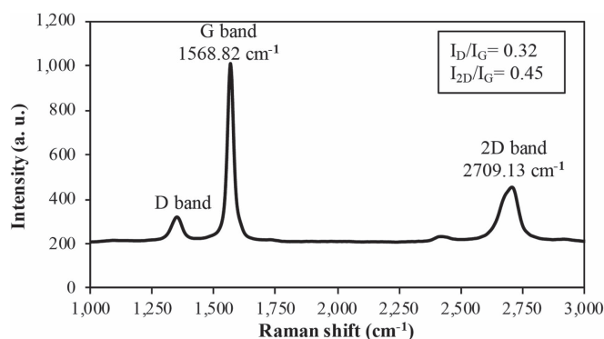
Figure 6. Raman spectrum of imprinted GNP on the fiber core.
