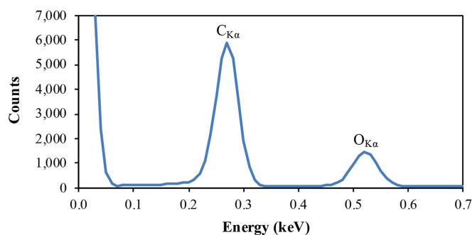
Figure 5. EDX spectrum of imprinted GNP on the fiber core.
