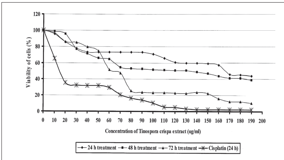
Figure 2. Percentage of viability of HepG2 against concentration of T. crispa aqueous extract.
