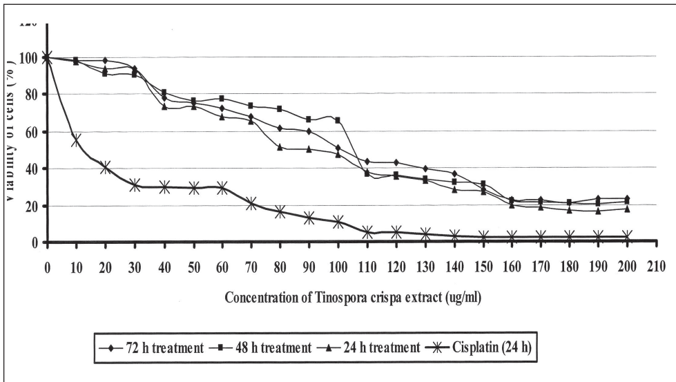
Figure 1. Percentage of viability of Caov-3 against concentration of T. crispa .
