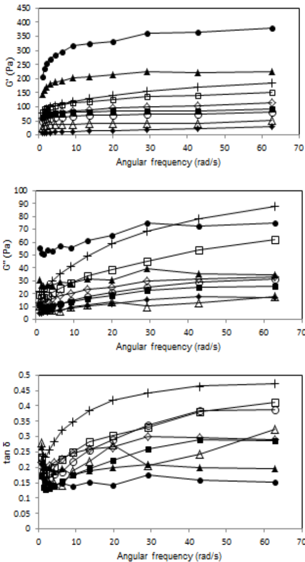
Figure 3. Variation of G' , G'' , and \tan \delta with angular frequency ((■) NCS, (●) NCS/XG, (+) NCS/Carrageenan, (□) NCS/HMP, (○) NCS/LMP, (▲) MCS, (▼) MCS/XG, (△) MCS/Carrageenan and (◆) MC/LMP
