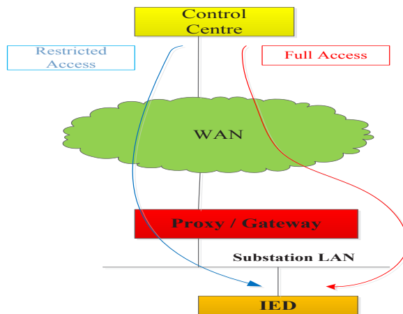
Figure 9. Proxy/gateway concept
