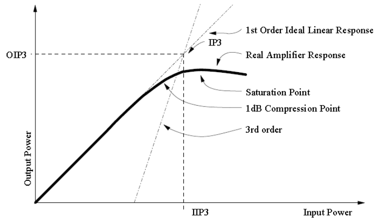
Figure 1.1: Inter-modulation Compression, and Saturation Points [2]
