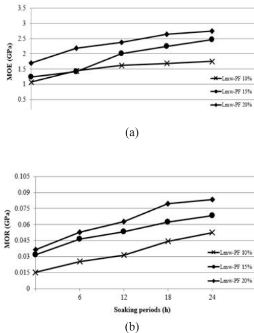
Figure 5. Static bending values of impreg OPW with different diffusion periods at different resin concentrations. (a) MOE (b) MOR
