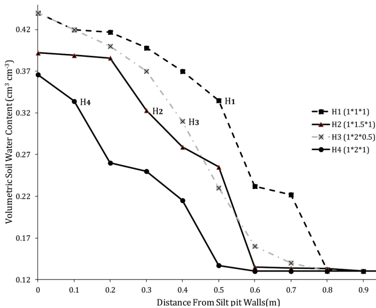
Fig.2: Volumetric soil water content at various horizontal distances from the silt pit walls. Soil water content at 0.50 m soil depth and at 72 hours.
