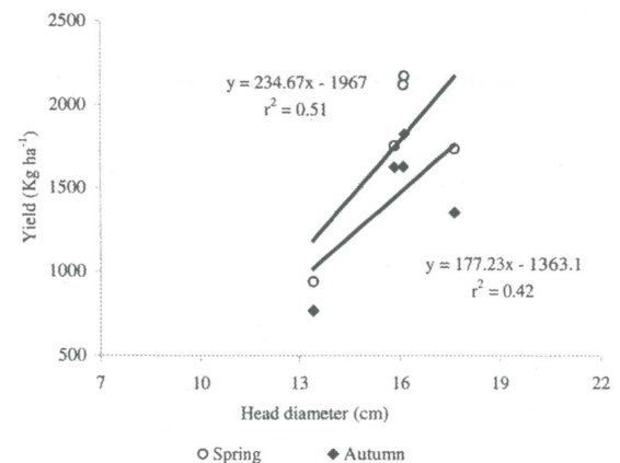
Fig. 3: Relationship between head diameter and seed yield
