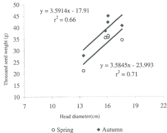
Fig. 1: Relationship between head diameter and thousand seed weight
