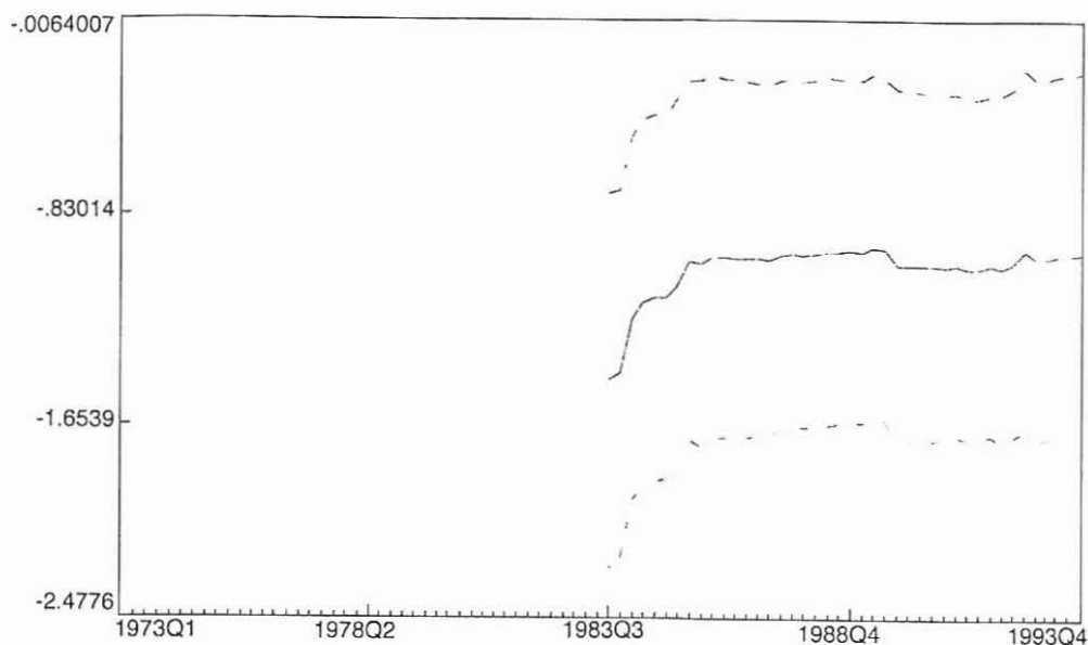
Fig. 2. Recursive estimates of the coefficient of \Delta ir , (Equation 6)
