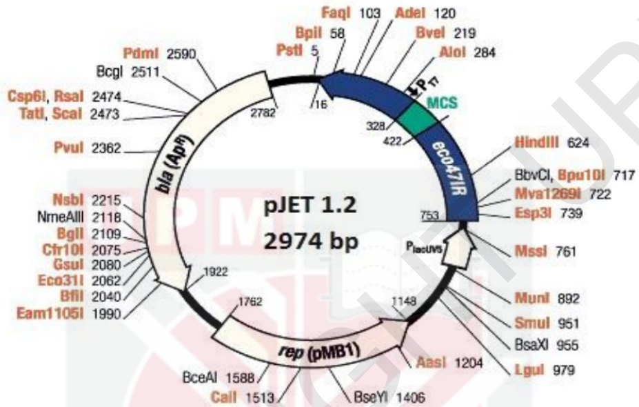
Map of pJET 1.2 cloning vector
