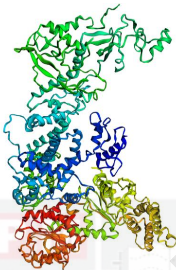
Figure 3.17 : 3D structure of Foc TR4 DCL proteins predicted by Phyre2
