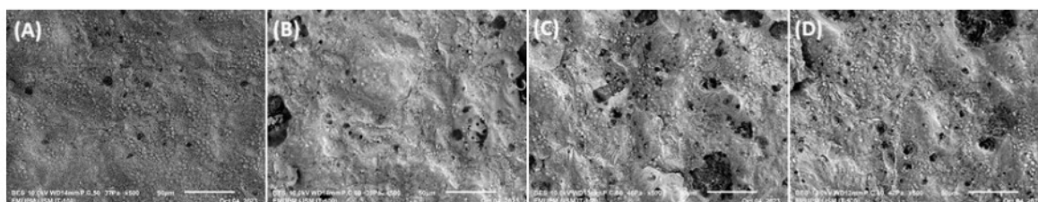
Fig. 4. Microstructure of PMCAs at magnification of x 500. Note: A = sample without starch, B = sample with rice starch of Putra 2 variety, C = sample with rice starch of NMR variety, D = sample with corn starch.
