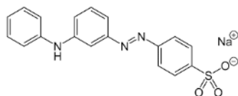
Fig. 1. Structure of Metanil Yellow.
