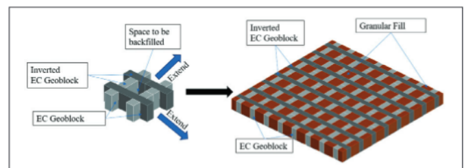
Figure 3: Installation of EC Geoblock
