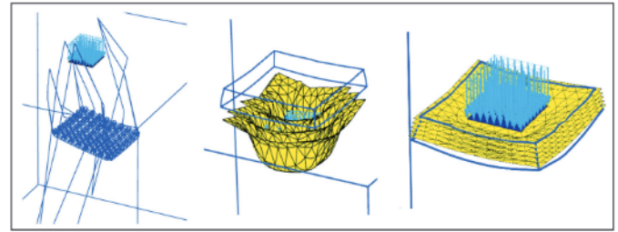
Figure 6: Failure behaviour of geogrid and EC Geoblock
