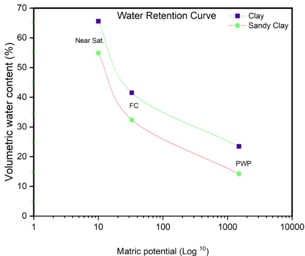
Figure 4. Soil retention characteristic curve for clay and sandy clay textured soils
