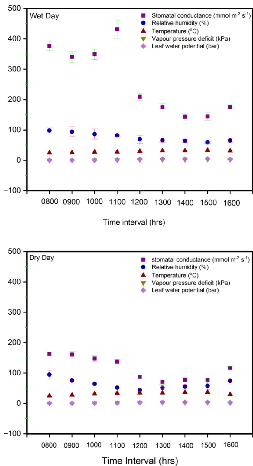
Figure 2. Diurnal pattern of the relative humidity, vapour pressure deficit and atmospheric temperature meteorological variables and stomatal conductance (STC) and leaf water potential (LWP) water stress indicators in wet and dry days
