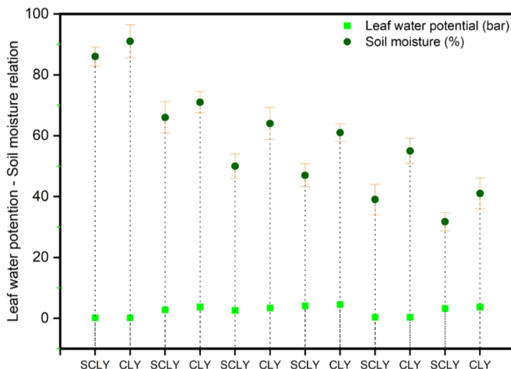
Figure 3. Relationship between soil moisture content and stomatal conductance and leaf water potential in oil palm tree in clay (CLY) and sandy clay (SCLY) textured soils
