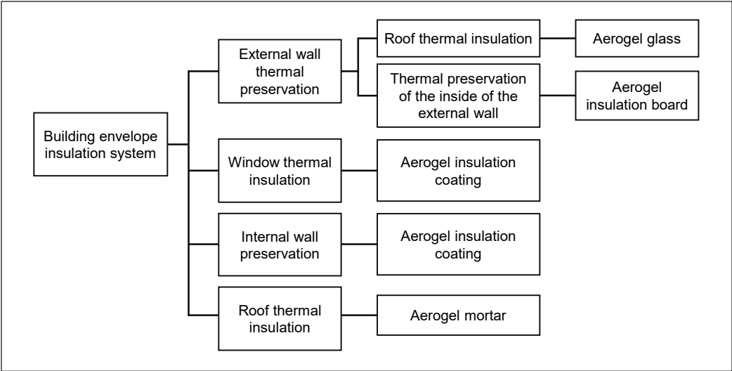
Figure 1. Building envelope insulation system utilizing aerogel material
