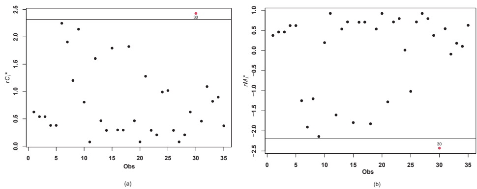
Figure 5. Index plot of adjusted Cox-Snell (a) and adjusted martingale (b) residuals for Hodgkin’s Disease data.
