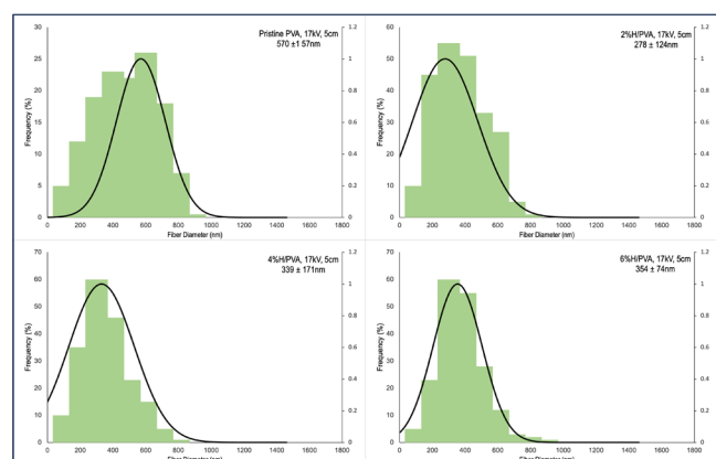
Fig. 4: Distribution of electrospun PVA fiber diameters with increasing Tualang honey concentration.
