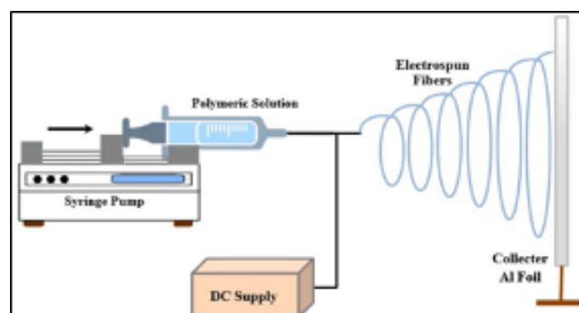
Fig. 1: Schematic diagram of electrospinning process to form nanofiber.
