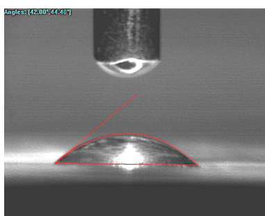
Fig. 2: An example of contact angle measurement using the VCA Optima Contact Angle Analyzer.
