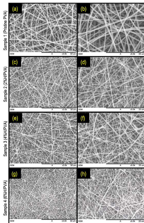
Fig. 3: SEM images at magnifications x3.0k and x5.0k of electrospun nanofibers: (a-b) Pristine PVA, (c-d) 2% honey/PVA, (e-f) 4% honey/PVA, and (g-h) 6% honey/PVA.
