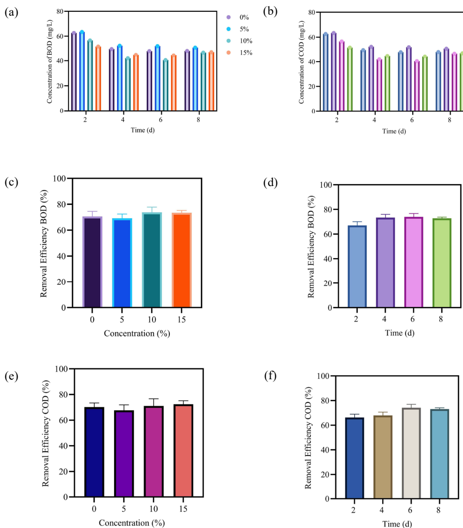
Fig. 6: (a)(b) BOD and COD concentrations, (c)(d)(e) BOD and COD efficiency.
