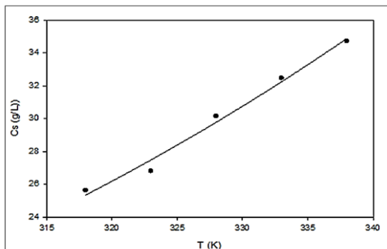
Fig. 16. Relationship between saturated extraction capacity, C and temperature for UAE of G. sepium leaves
