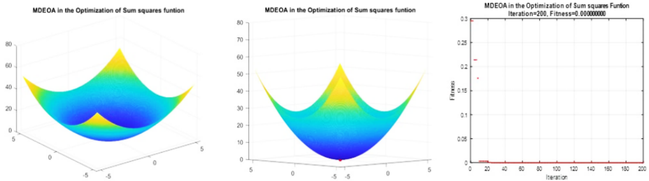
Fig. 23. The MDEOA in the optimization of Sum Squares function with the parameters as shown in Table 2
