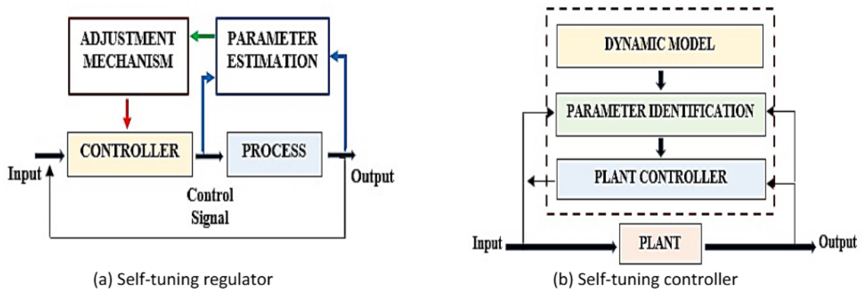
Fig. 2. Block diagram of a self-tuning regulator (a) and a self-tuning controller (b) [9]
