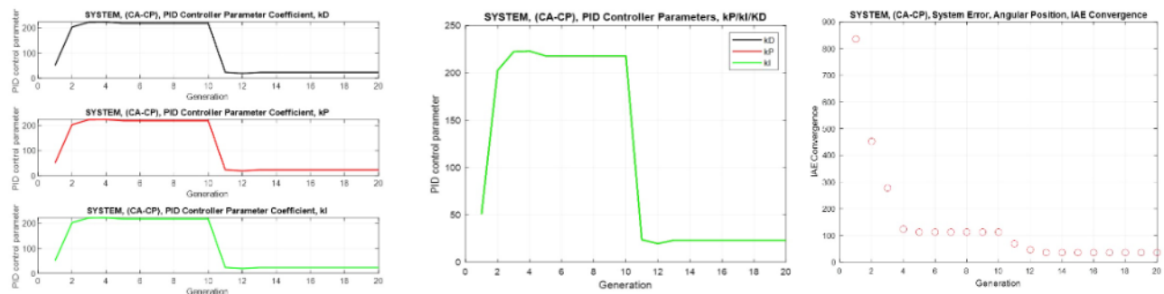
Fig. 32. The optimization results of MTRS for run test 2, with k_P=k_I=k_D=23.0551
