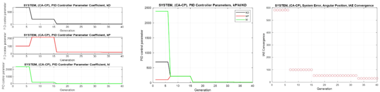
Fig. 34. The optimization results of MTRS for run test 4, with k_P=k_I=k_D=22.7323
