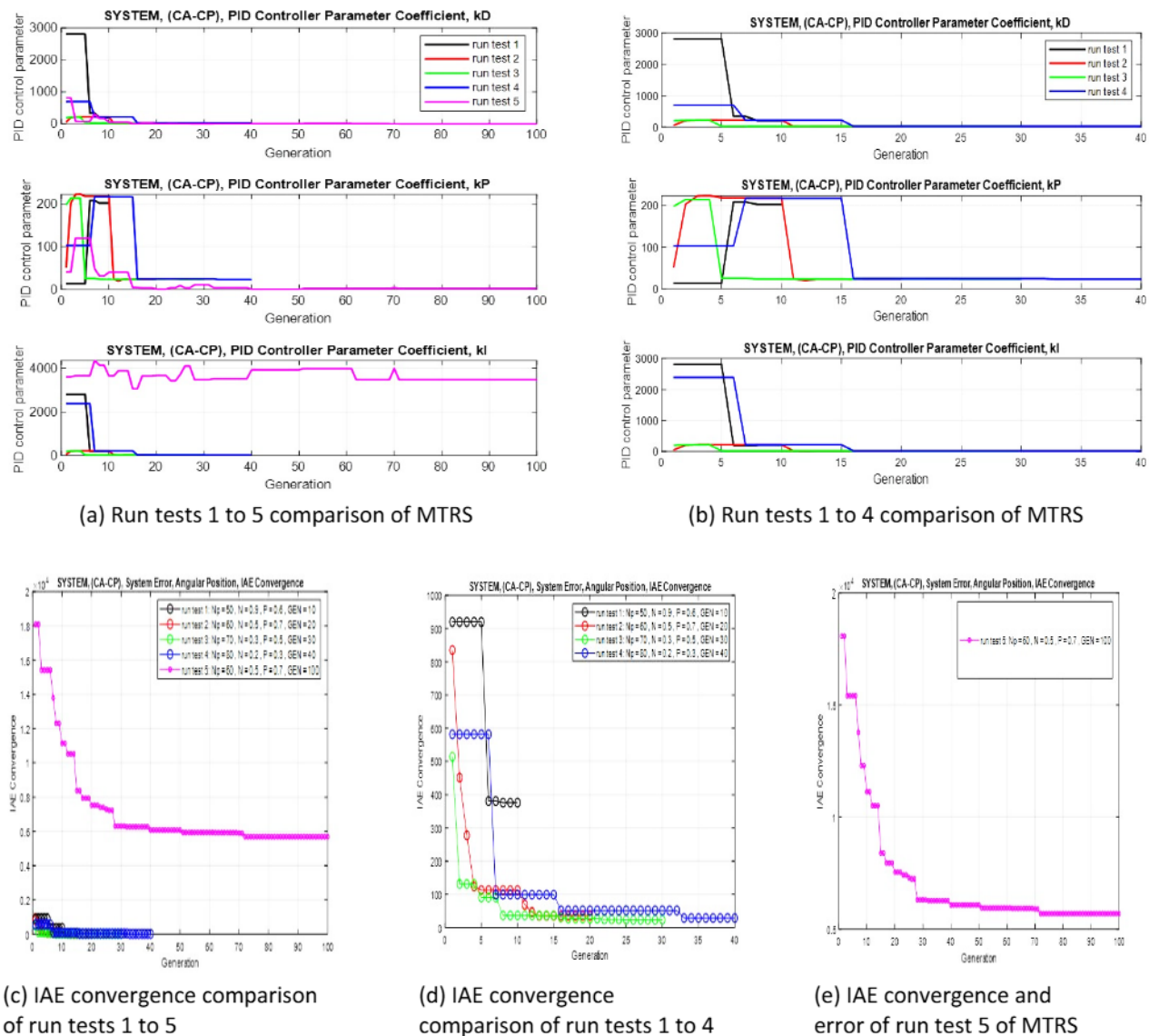
Fig. 36. The optimization run tests comparison results (a), (b), (c), (d) and (e) of MTRS
