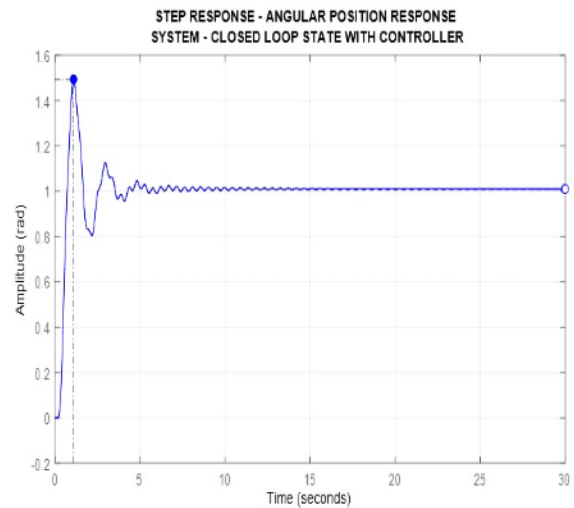
(f) Angular position response of closed loop system with controller
