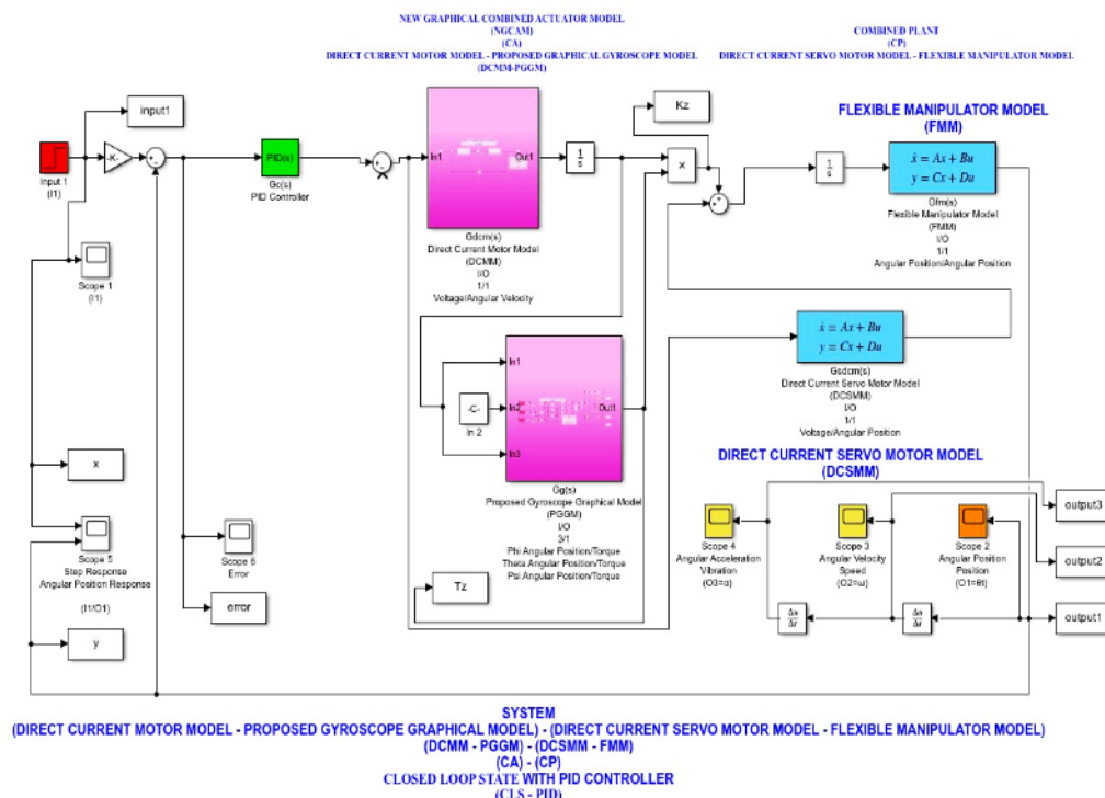
Fig. 29. The PID control block diagram simulation of MTRS
