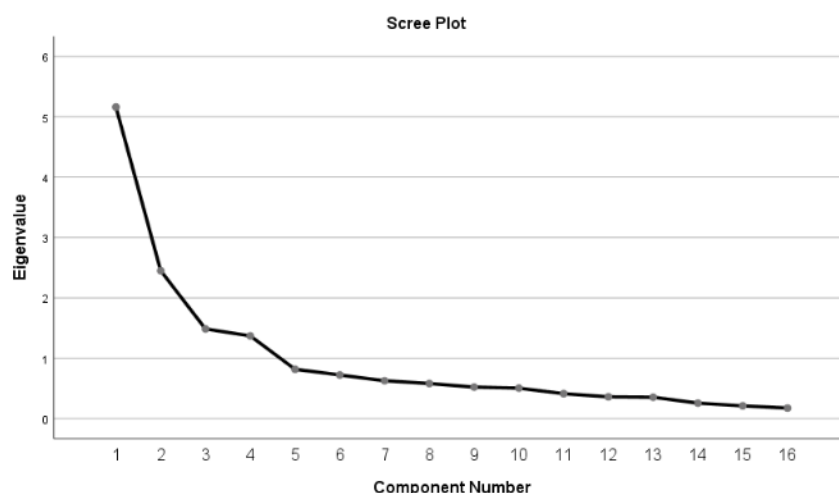
Figure 1. Scree Plot
