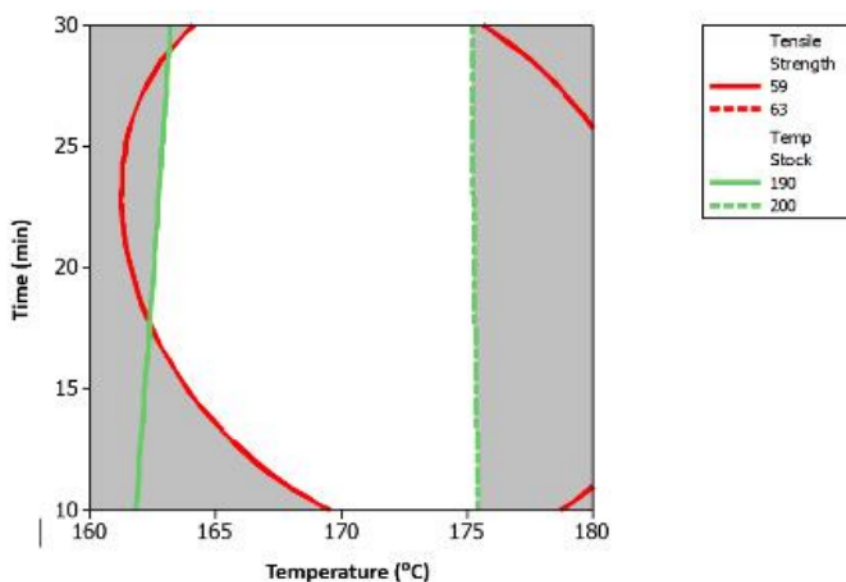
Figure 5. Overlay of tensile strength and stock temperature response.
