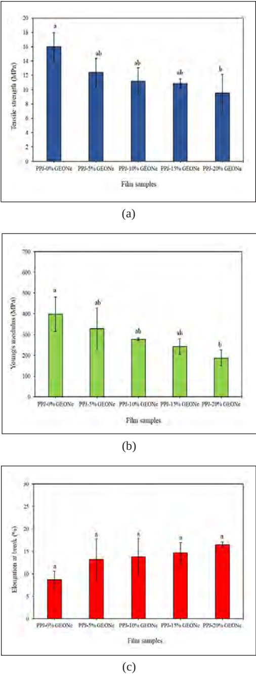
Figure 2. The tensile strength (a), Young’s modulus (b), and elongation at break (c) of PPJ-GEONE films. Note. Distinct letters (a, b, and c) show significant differences between means ( p \leq 0.05 ) when comparing different percentages of GEONE addition
