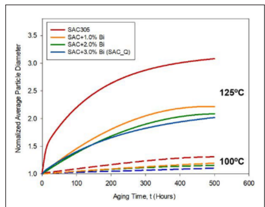
Figure 4. The normalized particle diameter of IMC particles at various conditions (Wu et al., 2021)
