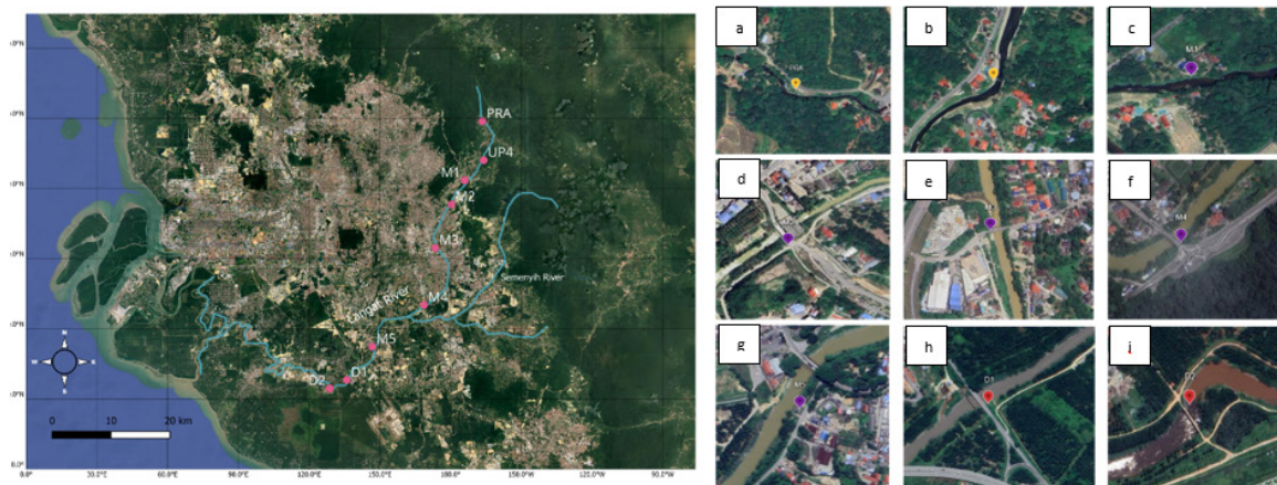
Figure 1 Map of Langat River in Peninsular Malaysia (left). The nine sampling sites and its land use types surrounding the river are depicted on the right
