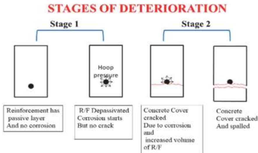
Figure 5. Stages of Deterioration due to corrosion in Reinforced concrete
