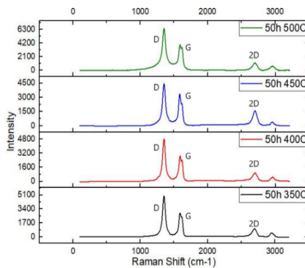
FIGURE 1. NDG for different annealing temperatures
