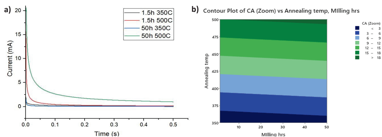
FIGURE 5. a) CA analysis for two-level factorial design and b) Contour plot of CA
