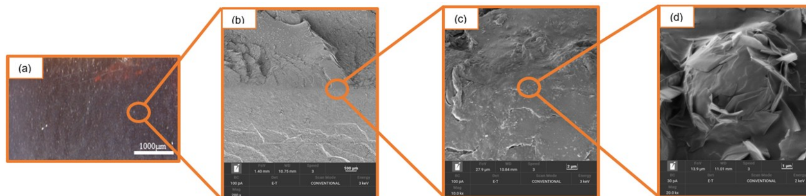
Fig. 7. Surface morphology of the welded vitrimer composite containing 4 wt.% activated carbon and 4 wt.% cellulose nanofibers.
