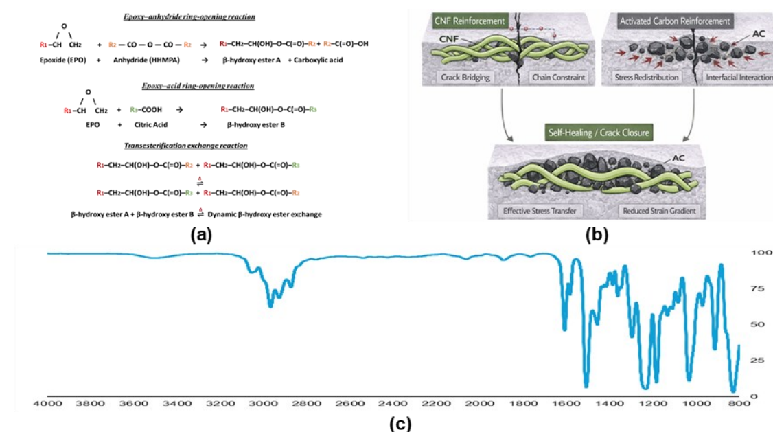
Fig. 8. (a) Chemical curing reactions illustrating the vitrimer bond exchange mechanism in the EPO system. (b) Mechanical reinforcement effects of NFC and activated carbon in the self-healing EPO-based composites. (c) FTIR spectrum of pure epoxidised palm oil (EPO)
