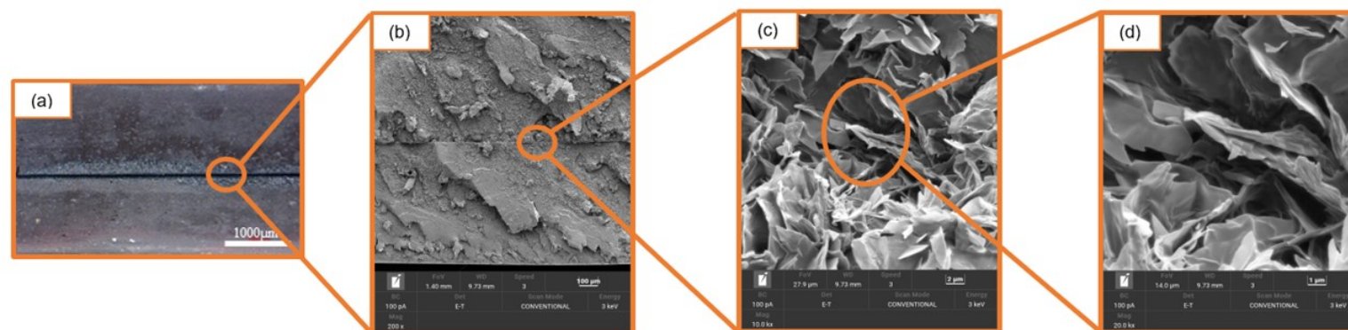
Fig. 6. Surface morphology of the welded vitrimer composite containing 4 wt% activated carbon.
