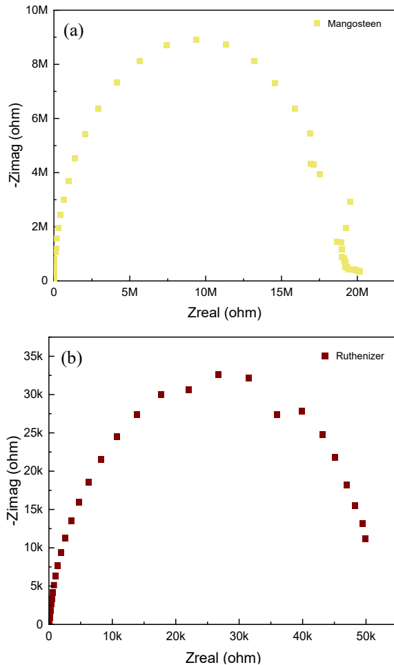
Fig. 7. (a) Nyquist plot for mangosteen dye DSSC, (b) Nyquist plot for Ruthenizer dye DSSC.
