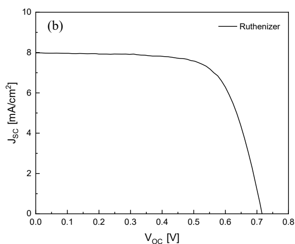
Fig. 4. (a) J – V characteristics curve of DSSCs based on different natural dyes, (b) J – V characteristics curve for Ruthenizer based DSSC.
