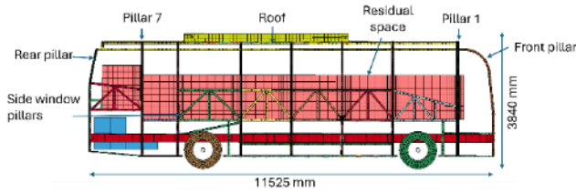
Figure 3 The bus model with the parts.
