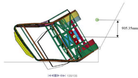
Figure 14 The vertical distance of CoG between starting and final position.
