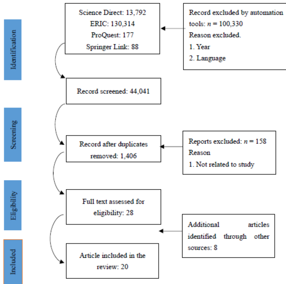
Figure 1. PRISMA flowchart.
