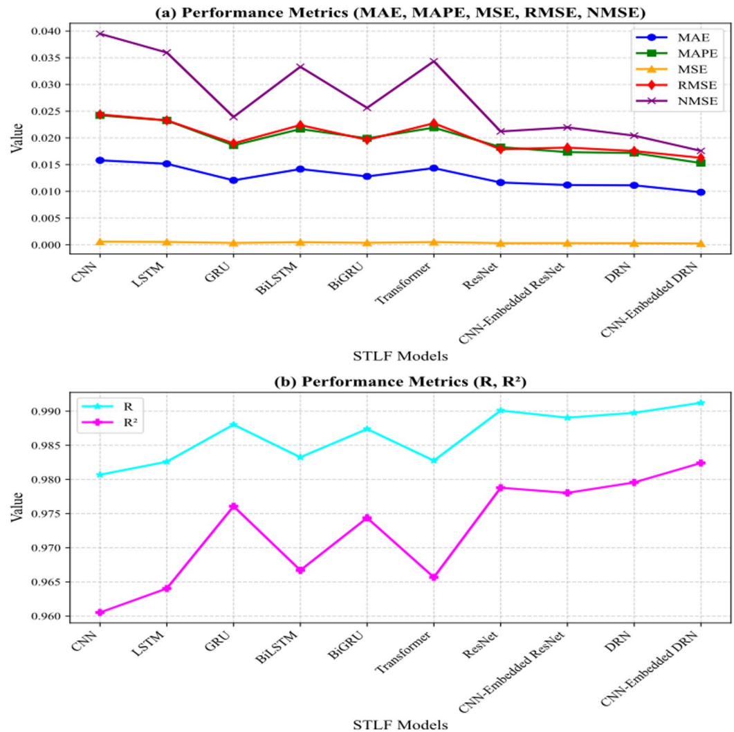
Fig. 8. A comparison between the proposed model and the baseline models in ISO-NE Dataset: (a) MAPE, RMSE, MAE, MSE, NMSE; (b) R and R 2 .
