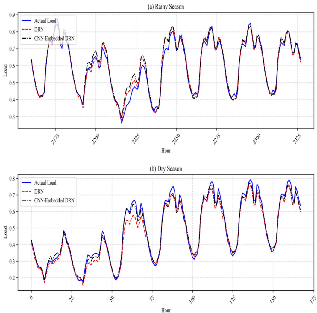
Fig. 11. The model’s performance on the Malaysia dataset for different seasons: (a) rainy, (b) dry (forecast values are normalized).
