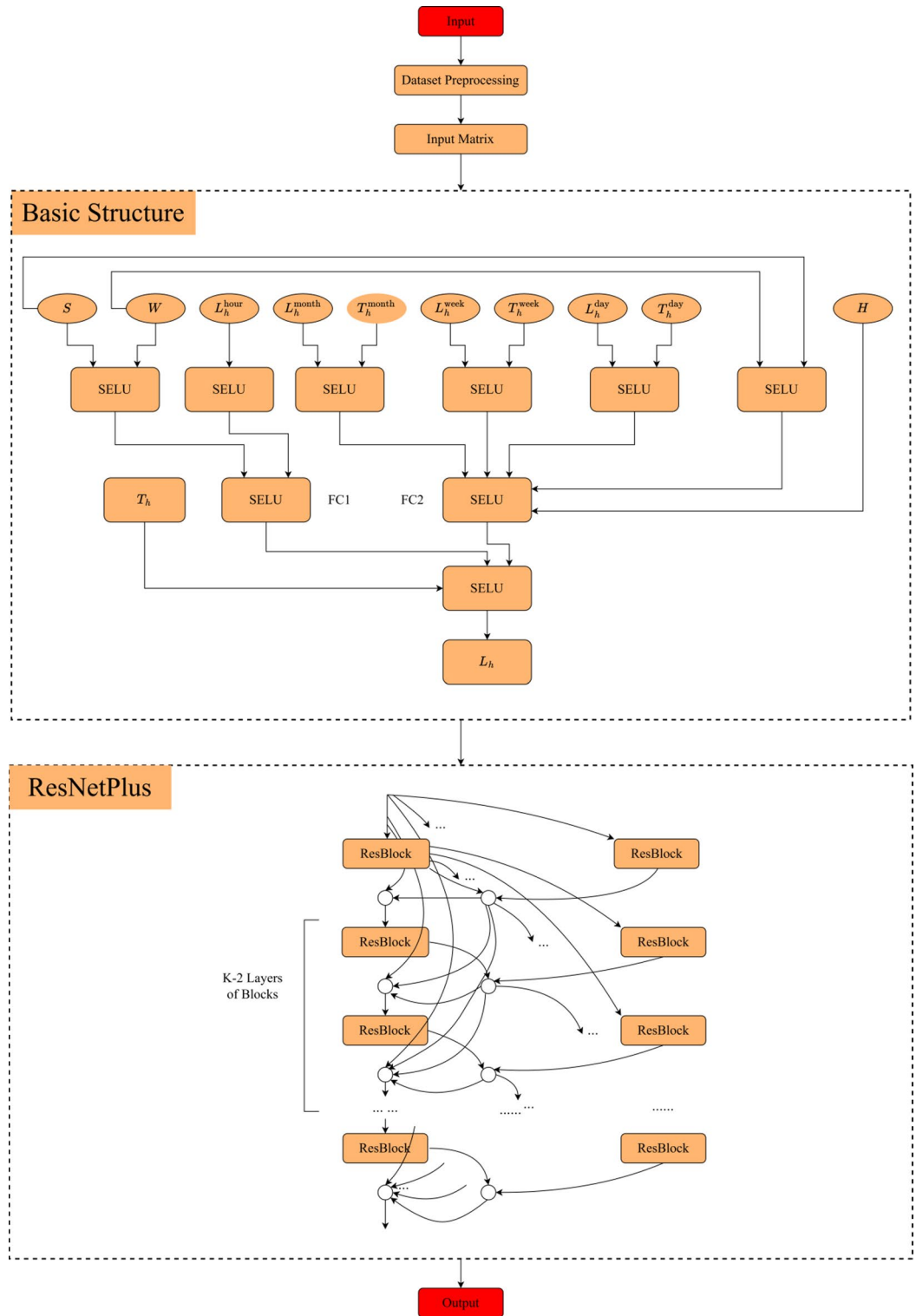
Fig. 2. The original framework 20 .
