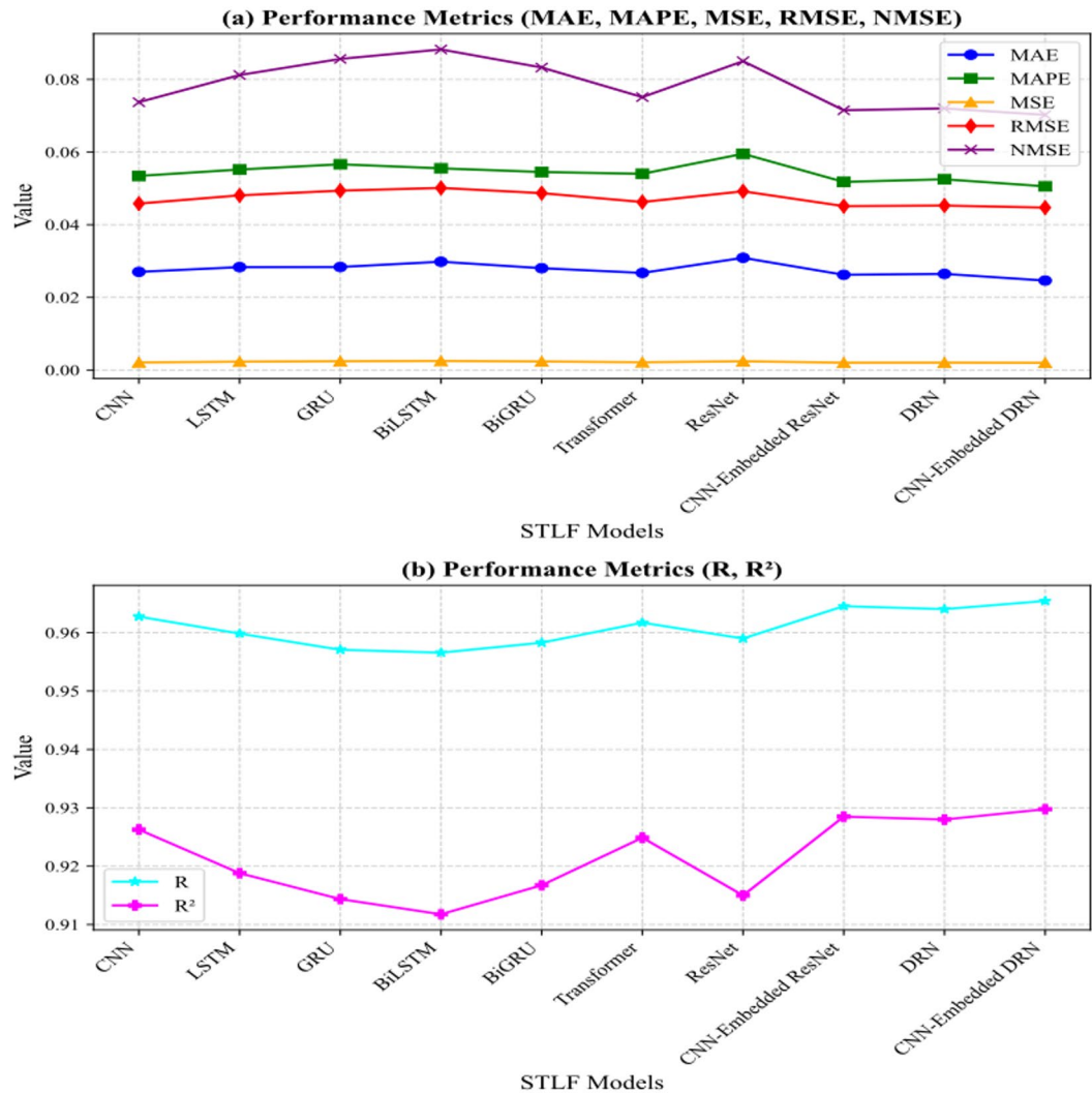
Fig. 9. A comparison between the proposed model and the baseline models in Malaysia Dataset: (a) MAPE, RMSE, MAE, MSE, NMSE; (b) R and R 2 .
