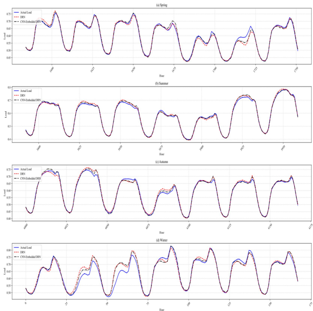
Fig. 10. The model's performance on the ISO-NE dataset for different seasons: (a) Spring, (b) Summer, (c) Autumn, and (d) Winter (forecast values are normalized).
