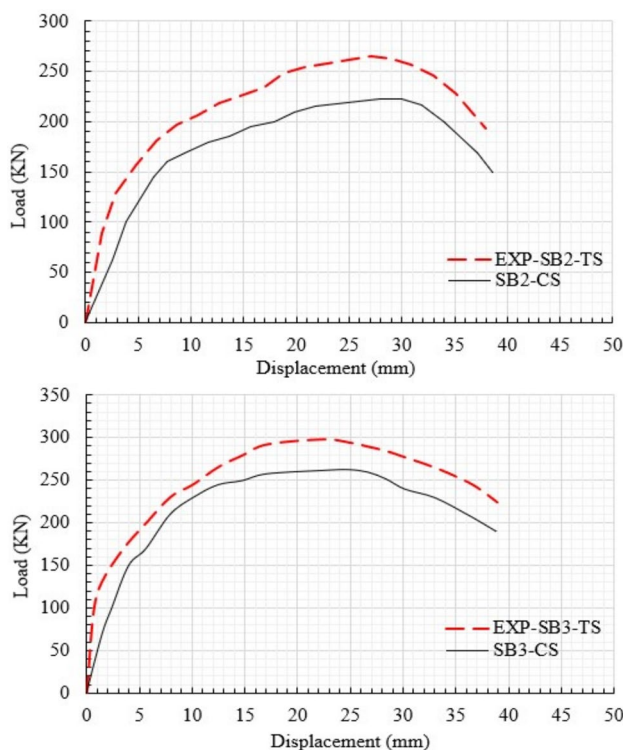
Fig. 20 Load–displacement relationship of models retrofitted on the compressive side
