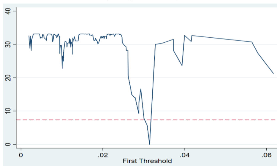
Figure 2: The Likelihood Function Plot
