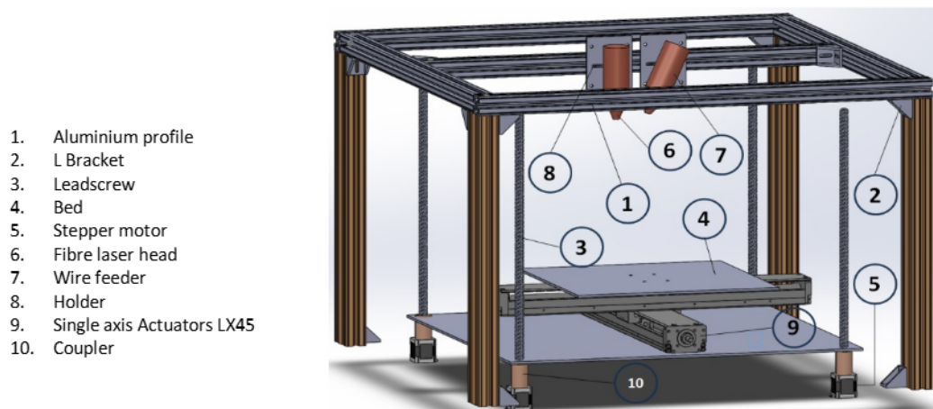
Fig. 1. The design of a 3D metal printer
