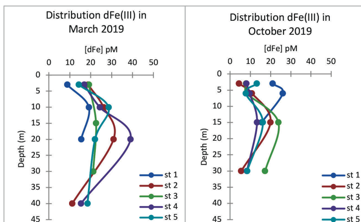
Figure 5: Concentration of dFe(III) in all stations during March 2019 and October 2019 at Pulau Redang, Terengganu
