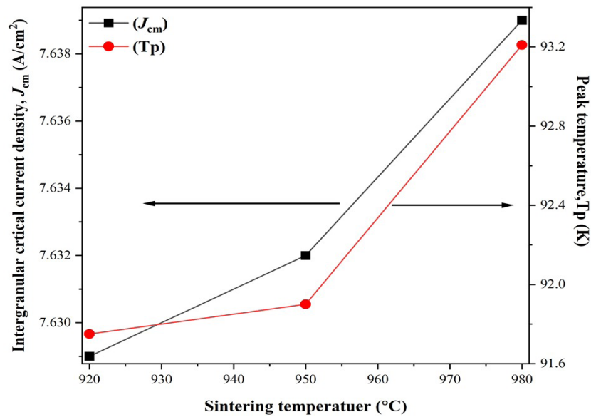
FIGURE 6. Variation of peak temperature ( T_p ) and intergranular critical current density ( J_{cm} ) for YBCO samples sintered at different temperatures. Solid lines are provided as visual guides only
