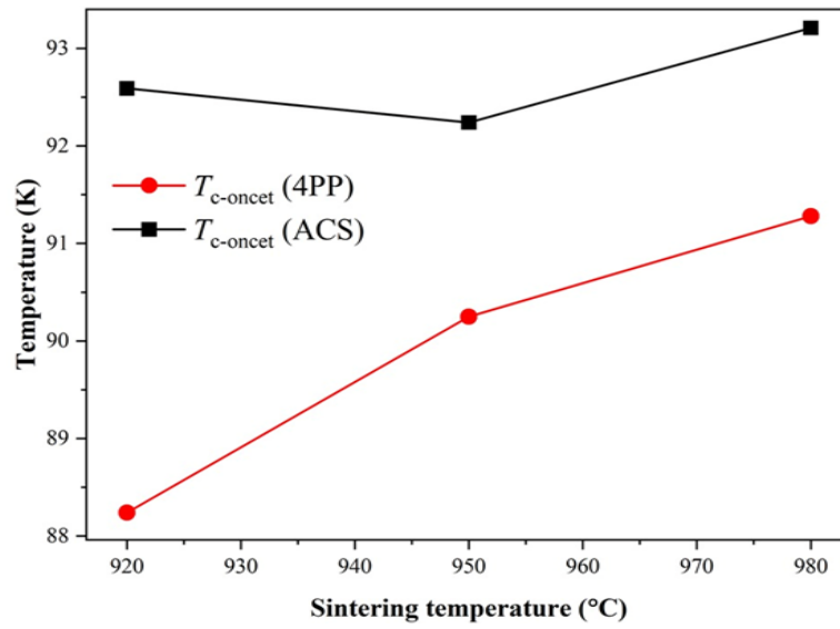
FIGURE 5. Shows the correlation between the critical temperature ( T_{c-onset} ) as measured by (4PP) and (ACS) techniques for YBCO samples sintered at different temperatures
