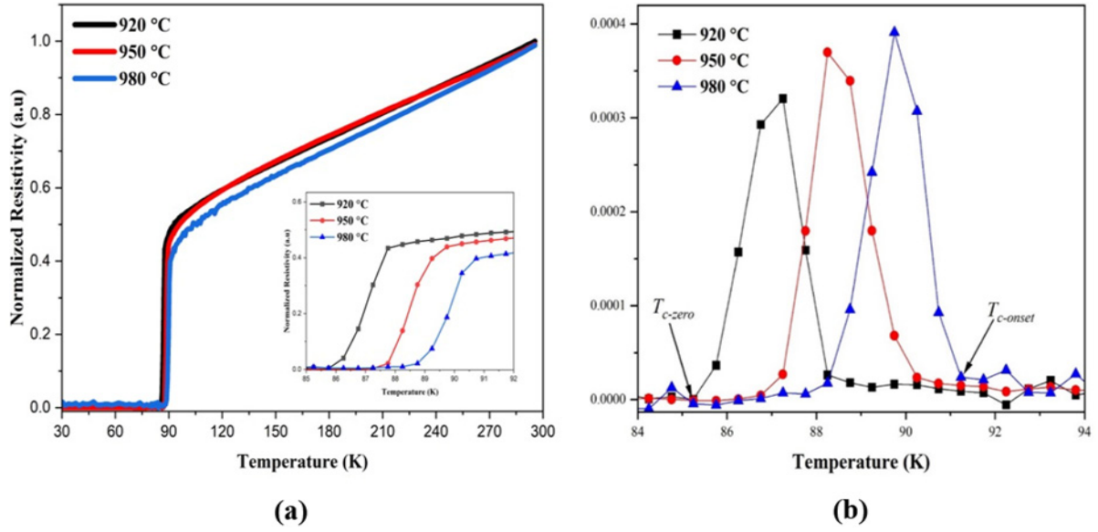
FIGURE 3. (a) Normalized resistance as a function of temperature for YBCO samples sintered at 920 °C, 950 °C, and 980 °C; (b) Temperature derivative of resistivity ( dp/dT ) for YBCO samples
