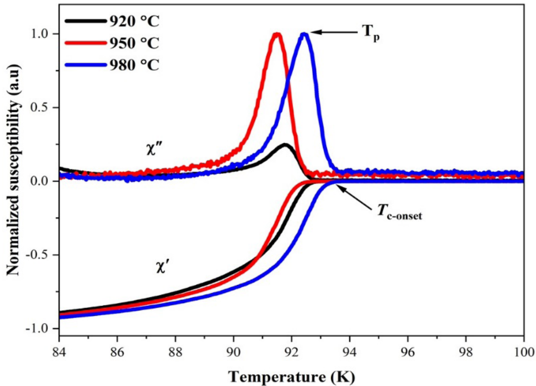
FIGURE 4. Presents the temperature-dependent AC susceptibility curves for YBCO samples sintered at different temperatures
