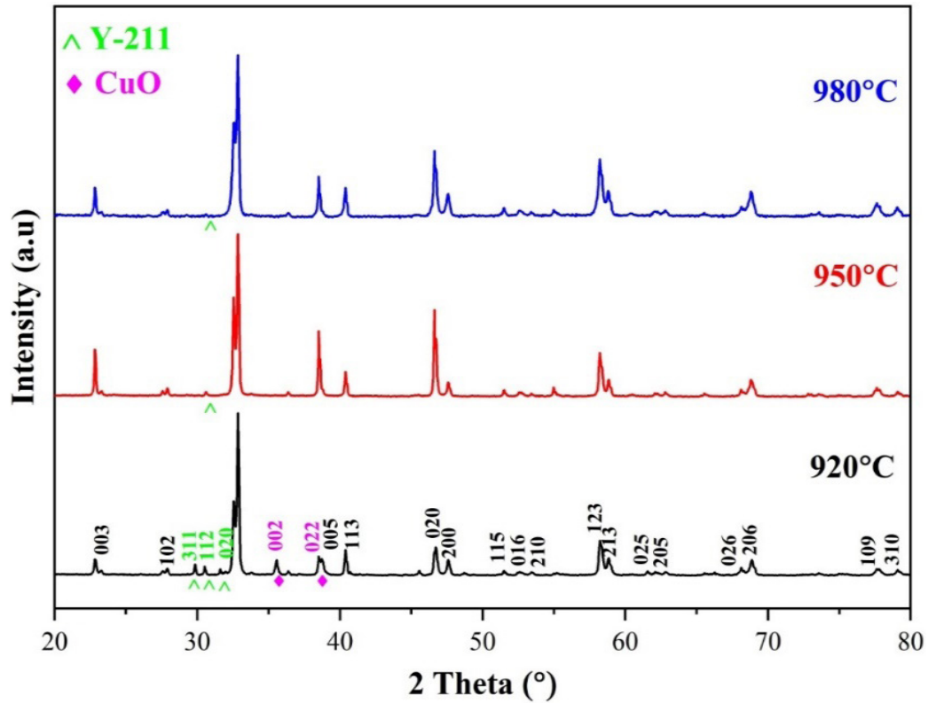
FIGURE 2. X-ray diffraction (XRD) patterns of YBCO samples sintered at 920 °C, 950 °C, and 980 °C
