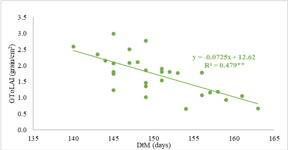
FIGURE 4. Linear regression analysis. The solid lines depict the regression between GToLAI and DtM. Regression equations and correlation coefficient (R 2 ) are included in the plot
