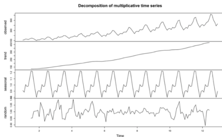
Figure 7: Decomposition Plot of the US Airline Passenger Data
