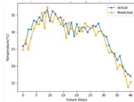
Figure 17. Forecasting Comparison for the Lowest MAPE Configuration of the Delhi Temperature Data
