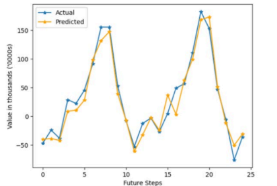
Figure 13. Forecasting Comparison for the Lowest MSE Configuration of the US Airline Passenger Data
