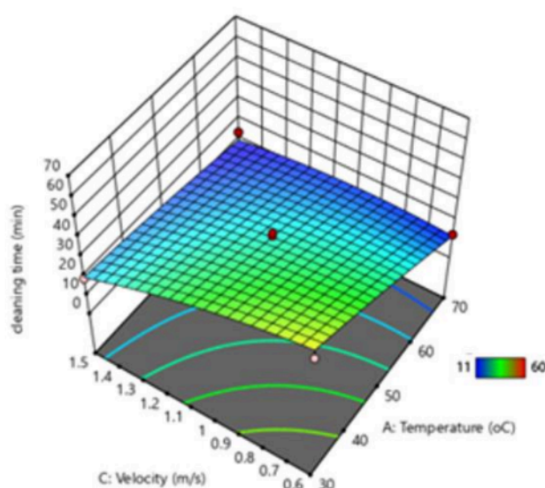
Figure 4. Response surface plot illustrating the cleaning time of milk fouling deposit influenced by the combined effects of fluid velocity and temperature.
