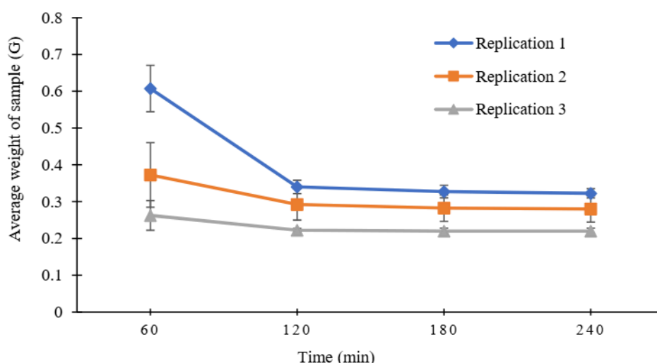
Figure 3. The average weight of the samples after baking at 90°C.
