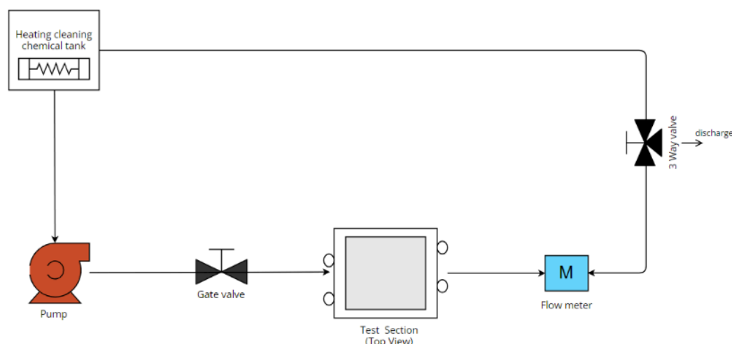
Figure 2. Process flow diagram of the cleanability experiments.
