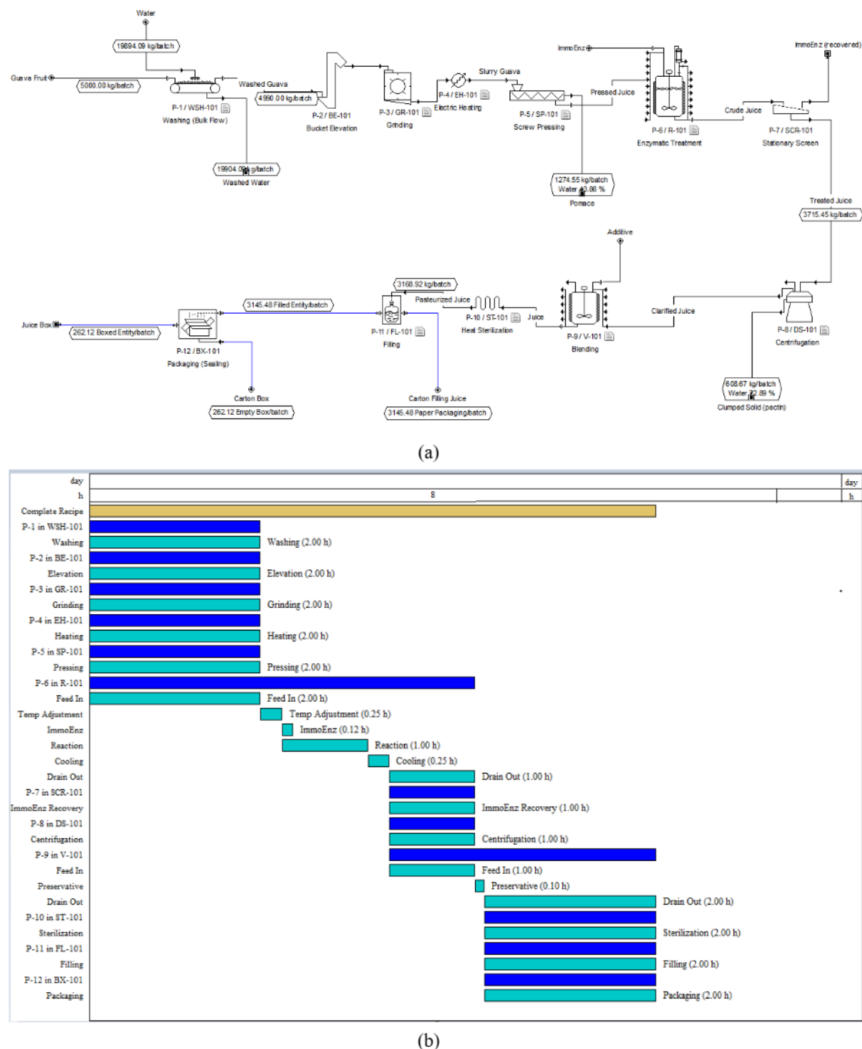
Figure 5. Proposed (a) SPD process flowsheet and b) operations Gantt chart of guava juice processing using immobilized pectinase (5000 kg guava fruit/batch)
