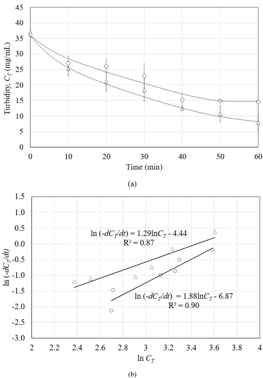
Figure 3. Profile of a) turbidity reduction and b) reaction kinetics study, ( \Delta native pectinase, \circ immobilized pectinase)
