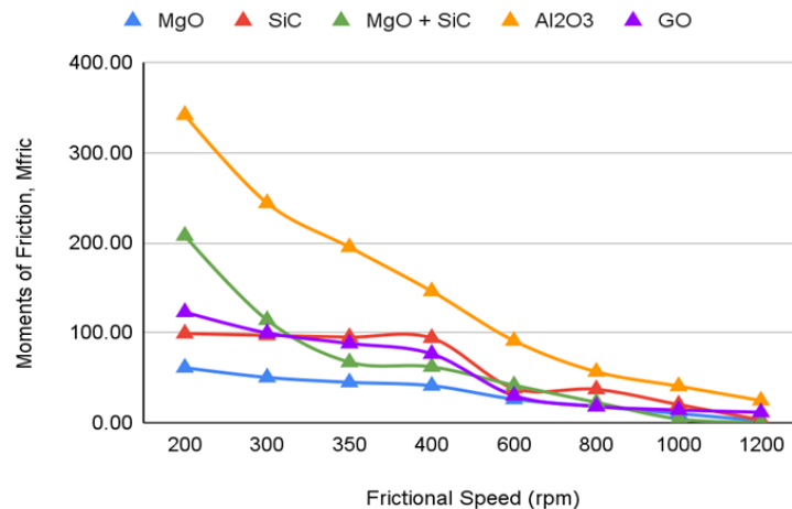
Figure 3: Moment of friction, M_{\text{fric}} as a function of rotational speed.
