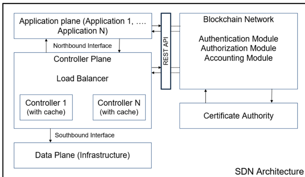
Fig. 5. The overview of experimental framework
