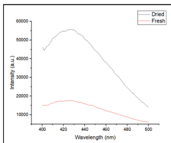
Figure 5. Emission scan of PL intensity of PM-AgNPs
