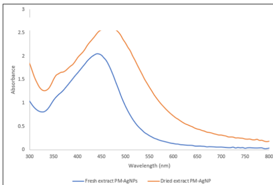
Figure 2. UV-vis absorbance spectrum of fresh and dried PM-AgNPs
