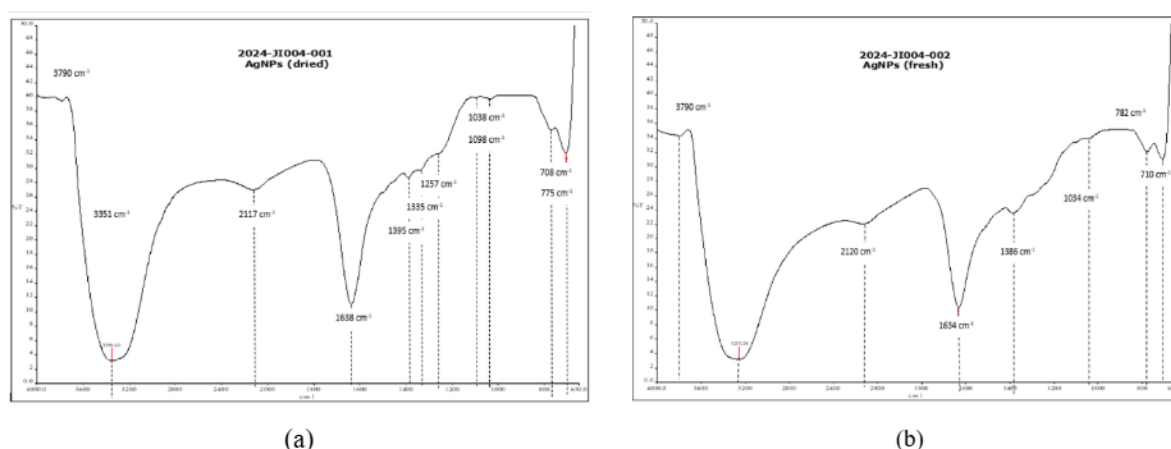
Figure 3. Infrared spectra of FTIR analysis. (a) dried extract (b) fresh extract
