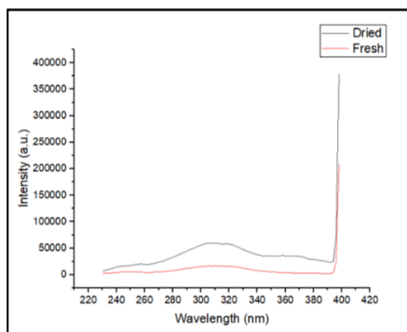
Figure 4. Excitation scan of PL intensity of PM-AgNPs
