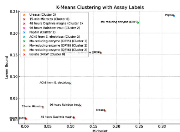
Fig. 4. K-Means clustering of enzyme assays based on IC 50 values (lower bound and midpoint) under mercury exposure.
