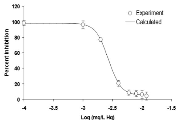
Fig. 2. Fitting mercury inhibition to the Mo-reducing enzyme of using the log(inhibitor) vs. response with variable slope. Data is mean \pm standard error ( n=3 ).
