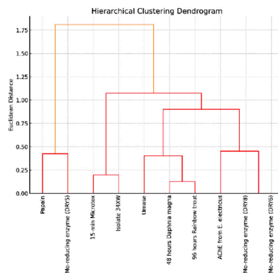
Fig. 3. Hierarchical Clustering Dendrogram of enzyme assays based on IC_{50} values (lower bound and midpoint) under mercury exposure.
