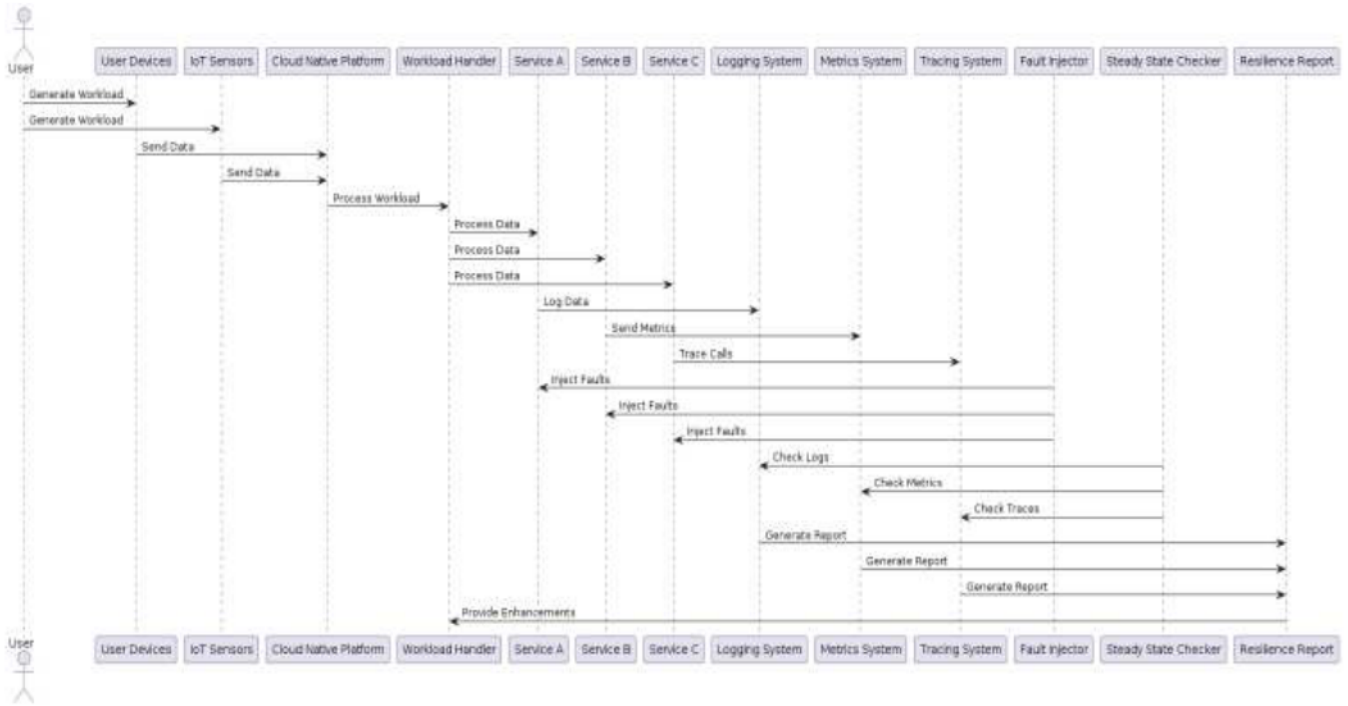
Fig. 4 Sequence Diagram
