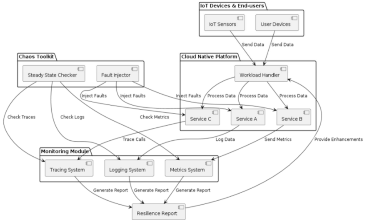
Fig. 1 The Architecture of the Proposed Chaos Engineering Tool
