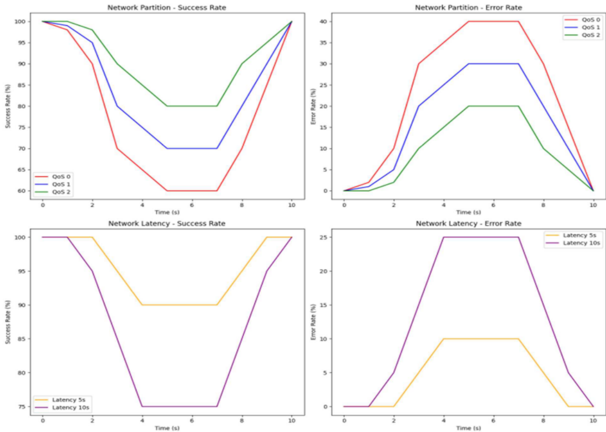
Fig. 8 Line graph of the result of cloud provider fault injection experiment
