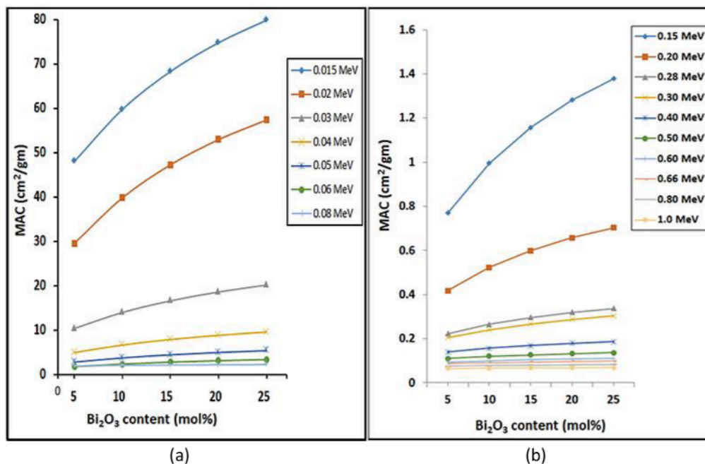
Fig. 3. MAC variation of photon energies (a) Lower (b) Intermediate
