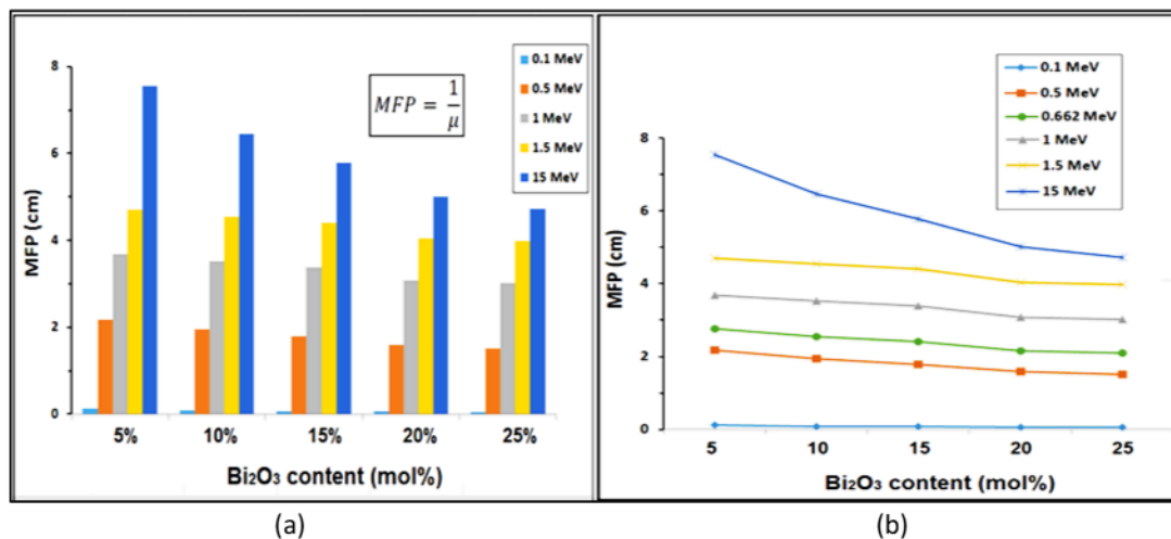
Fig. 6. (a) MFP analysis for the five glass samples at selected photon energies (b) Variation of MFP trends as bismuth content changes
