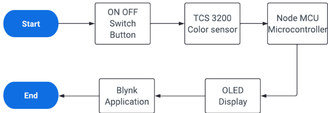
Fig. 1. Block diagram of MaizeMeter
